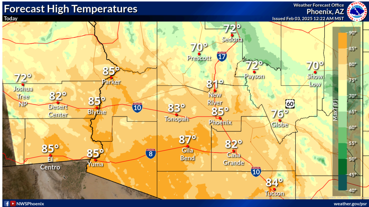
MaxT_Today.png
