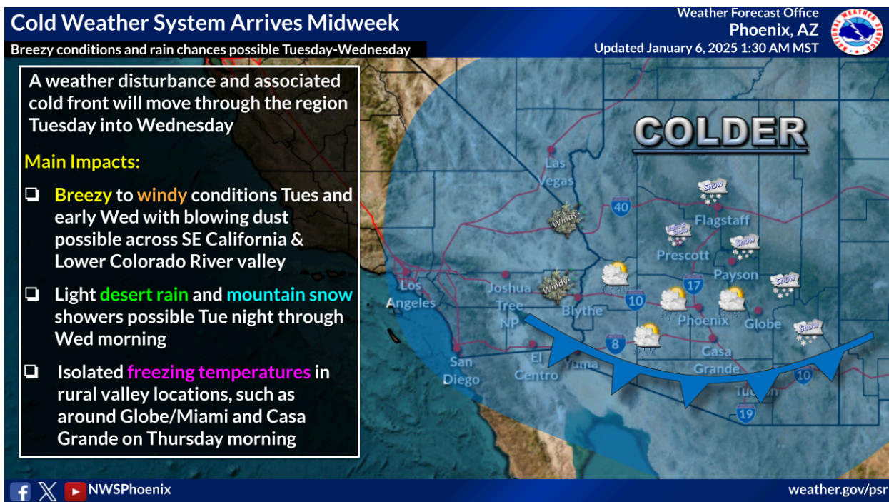
25-01-06 Weather System.png
